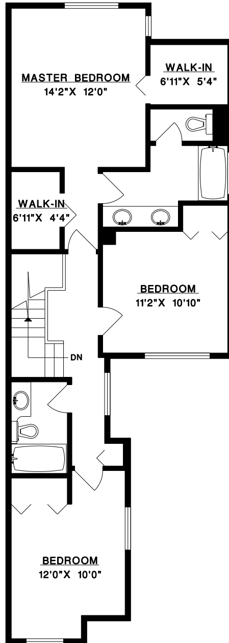
UPPER FLOOR
