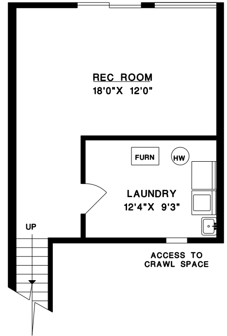
LOWER FLOOR
